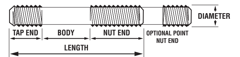
Tap-End Studs
