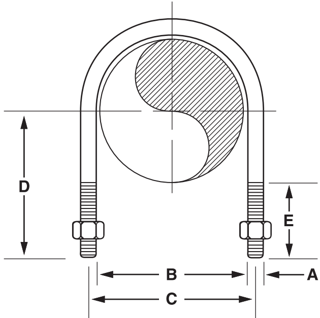
Figure 120 U-Bolt
