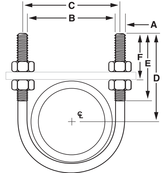
Figure 137 U-Bolt
