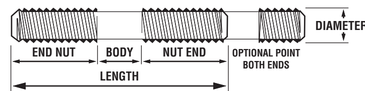
Double-End Studs
